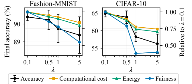
Fig. 3. Sensitivity to the cost trade-off \lambda on Fashion-MNIST (left) and CIFAR-10 (right). The black curve is accuracy. Computational cost, energy consumption, and fairness are normalized to their \lambda = 0.1 values. The trade-off is mild on Fashion-MNIST and sharper on CIFAR-10.
